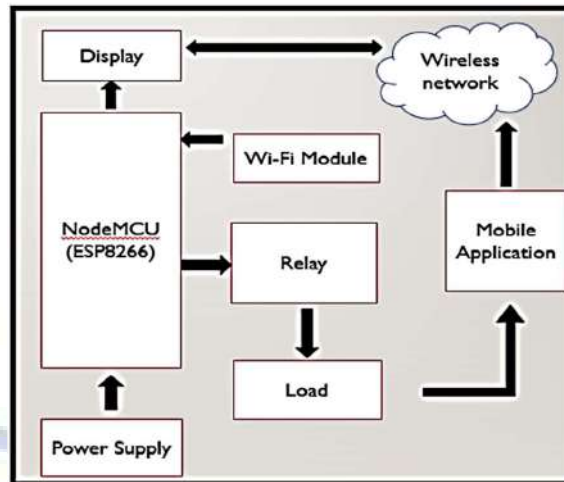
Figure 23: Schematic Diagram of The Developed System
