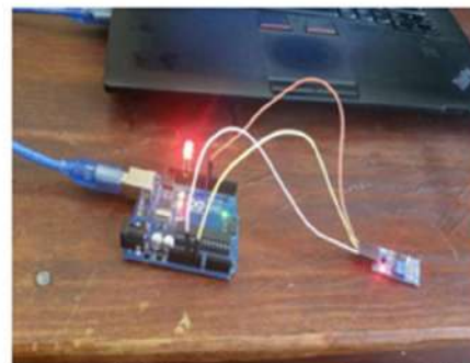
Figures 29 and 30: Showing the Photosensitive Sensor Module Connection – Day Ligh ON, Photosensitive Sensor Module Connection – Day Light OFF respectively.
