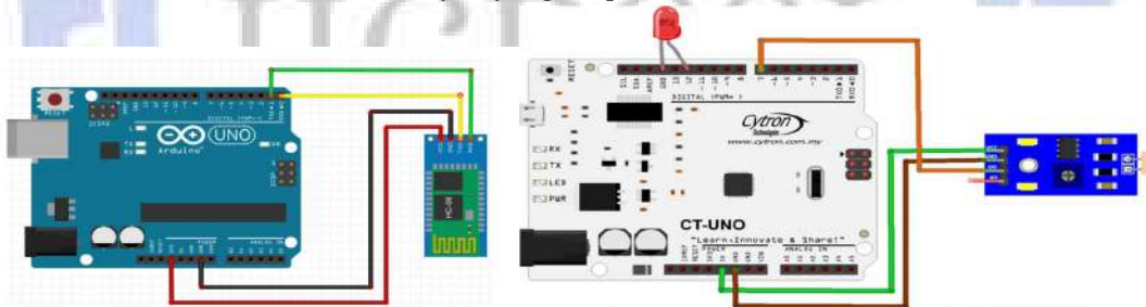
Figures 27 and 28: The Arduino Uno Connected to Bluetooth Module (HC-06) & Photosensitive Sensor Module Connection respectively.
