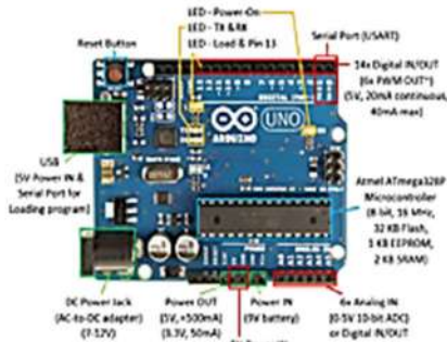
Figure 14: The Arduino Uno Board
