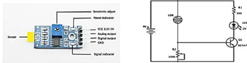
Figure 19: Photosensitive Sensor Module & Schematic Diagram
