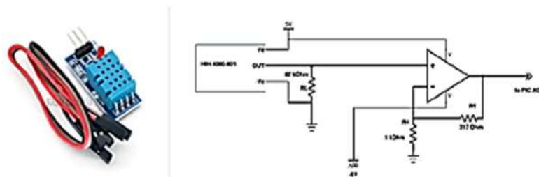
Figure 21: DHT-11 Digital Temperature and Humidity Sensor and Schematic Diagram
