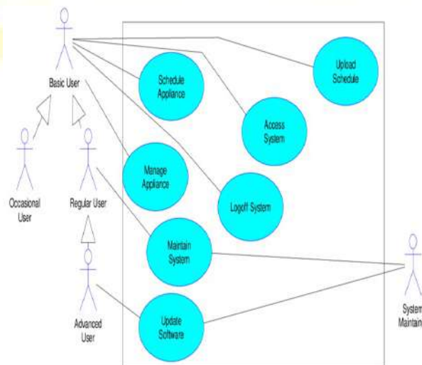
Figure 22: Use Case Diagram of the Developed System
