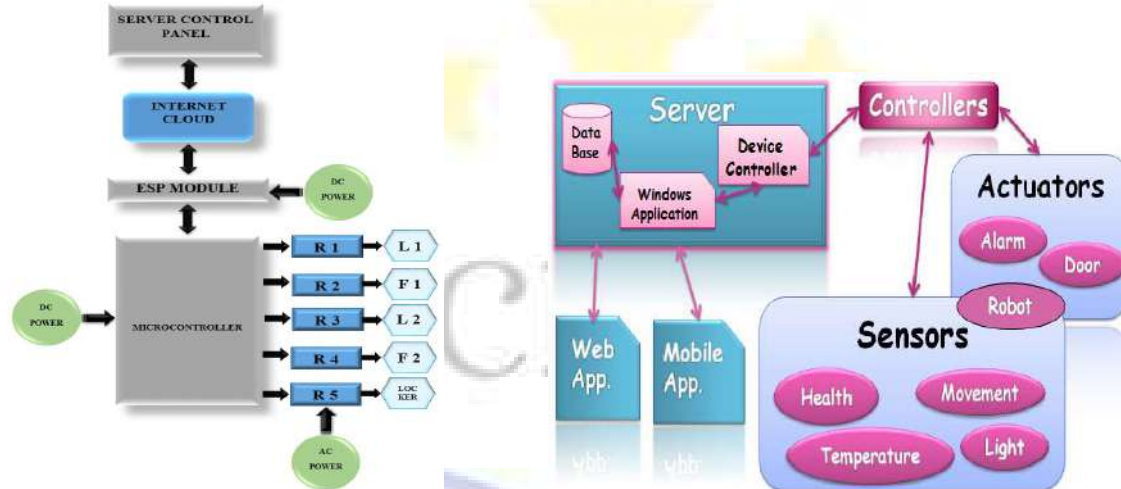
Figures 6 and 7: Schematic Diagram for IOT Based Home Automation System & State Diagram of the Intelligent Controlling System respectively.
