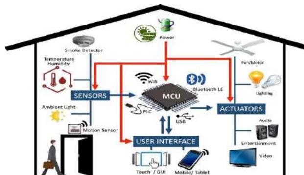
Figure 4: Overview of Intelligent Home Automation System Showing Devices Connected
