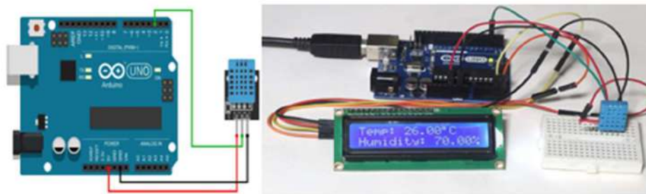
Figures 33 and 34: DHT11 Sensor Module Connection & DHT11 Sensor Module Connection – Active respectively.
