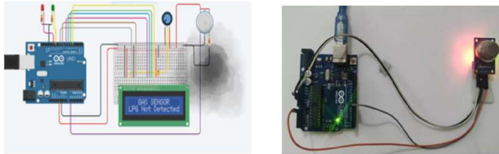
Figures 31 and 32: MQ-2 Smoke, Gas Sensor Detector Connection – Active & MQ-2 Smoke, Gas Sensor Detector Connection respectively.
