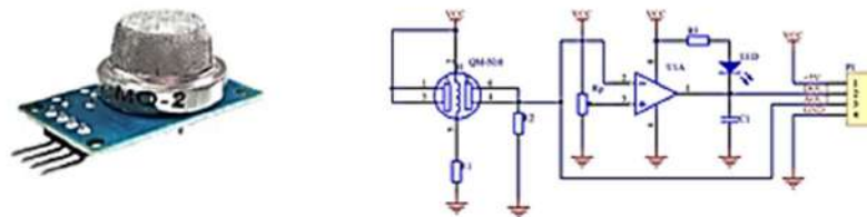
Figure 20: ADIY MQ2 Smoke/Gas Sensor Module & Schematic Diagram
